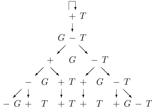
Figure 9: A folding tree with G s, T s and signs.
