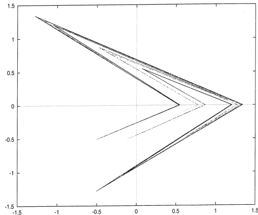
Figure 1: The Lozi attractor for a = 1.7 and b = 0.5 .
