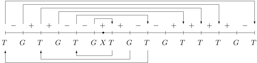
Figure 6: The action of the map on the folding pattern with signs.
