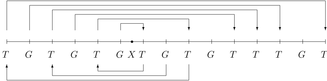
Figure 5: The action of the map on the folding pattern.
