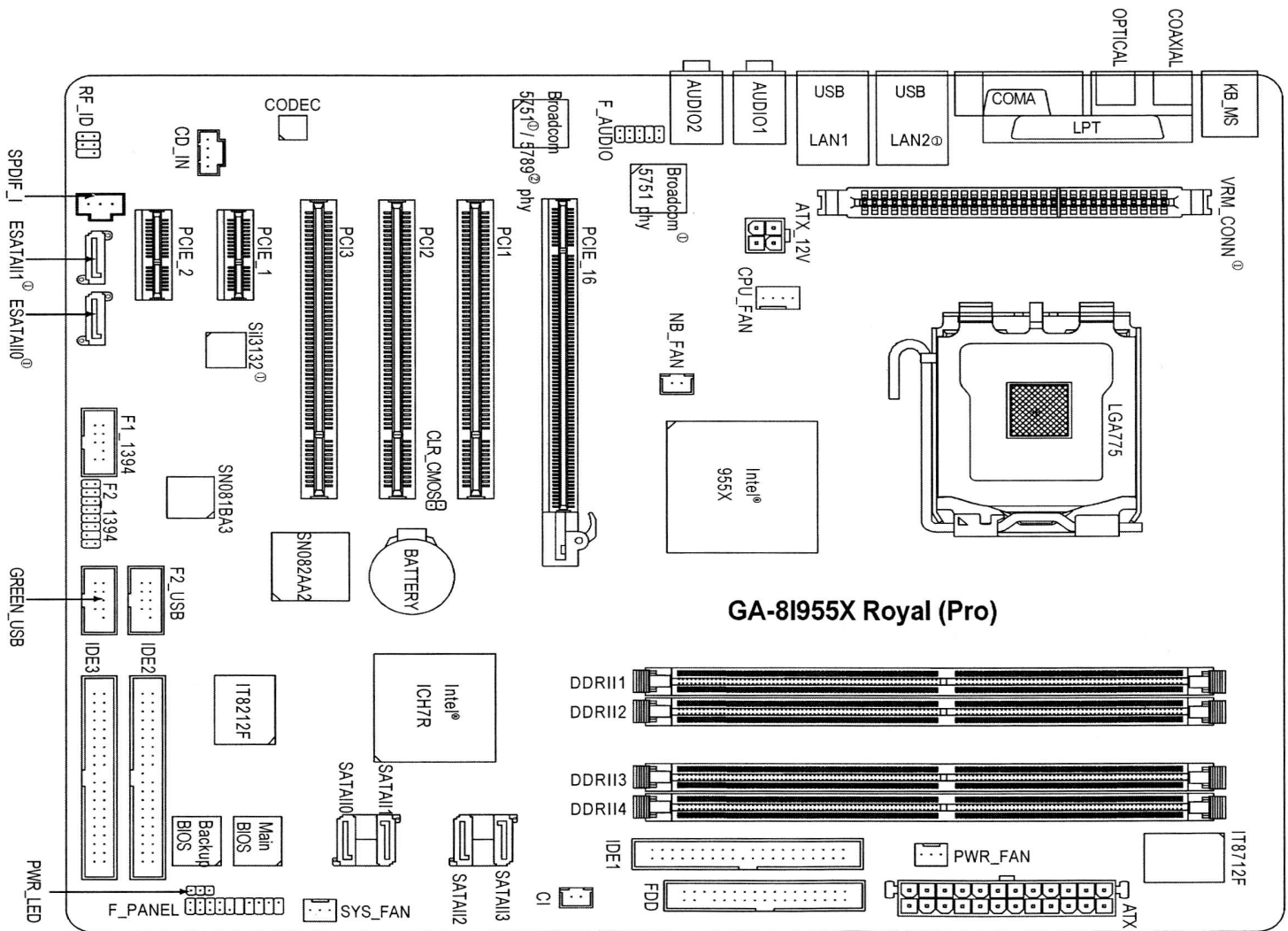
GA-81955X Royal/GA-81955X Pro Motherboard Layout
