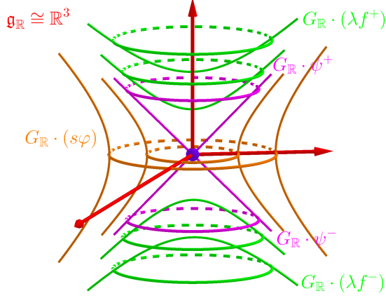
FIGURE 2. Adjoint orbits for SL_2(\mathbb{R}) .
