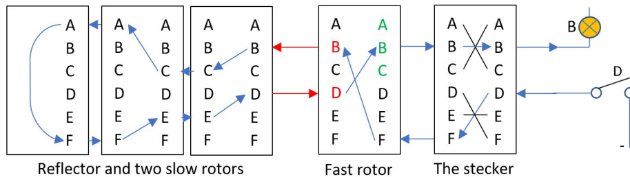
FIGURE 2. A military Enigma with a stecker.
