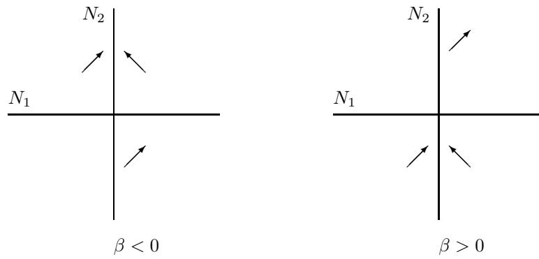
Figure 3 : \delta = 0
