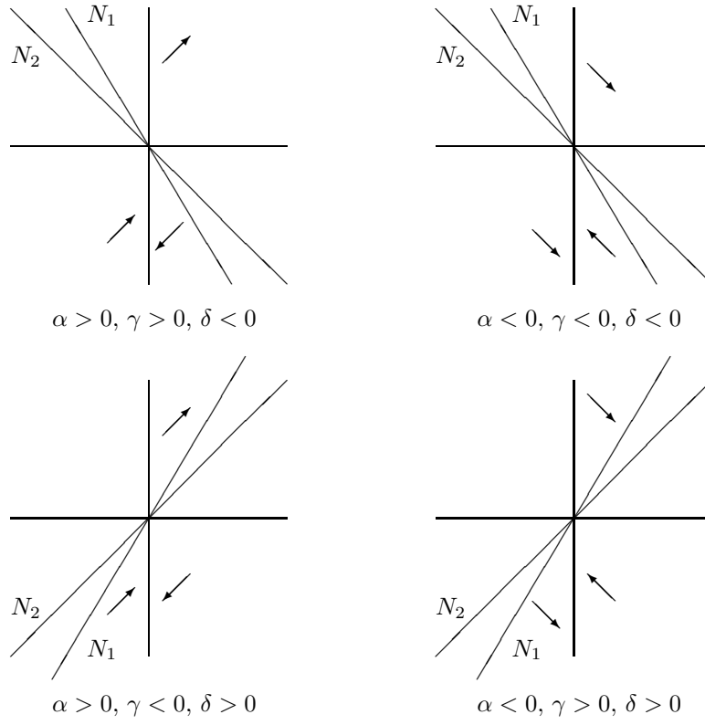
Figure 2 : \beta > 0
