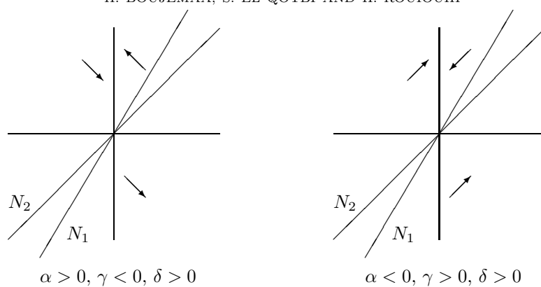
Figure 1 : \beta < 0
